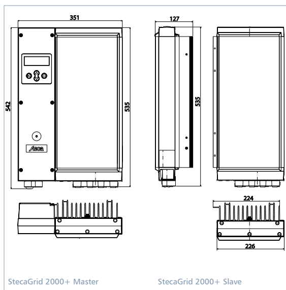
StecaGrid 2000+ Master
